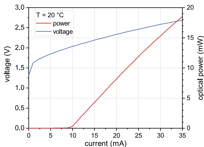
Typical PI and VI curve of a nanoplus FP laser at 761 nm
