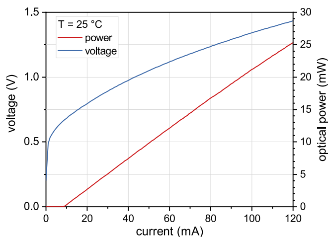
Typical PI and VI curve of a nanoplus FP laser at 2330 nm
