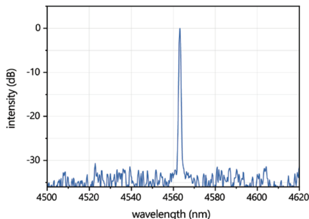
Typical room temperature cw spectrum of a nanoplus DFB laser at 4565 nm
