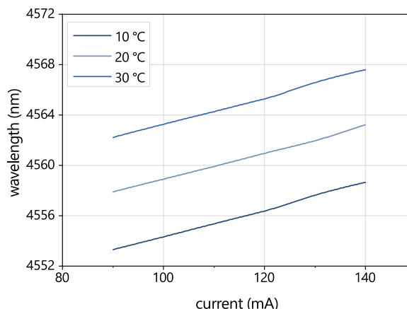
Typical mode hop free tuning of a nanoplus DFB laser at 4565 nm by current and temperature
