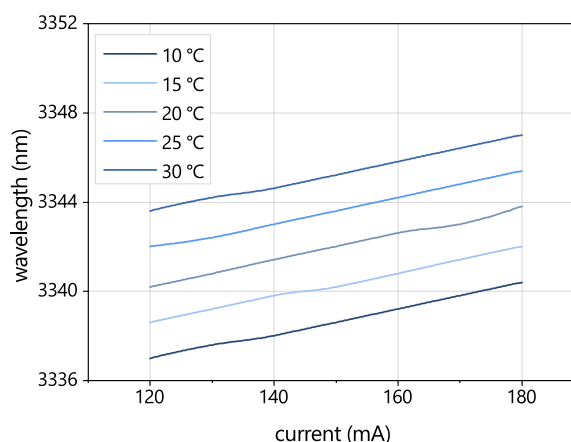
Typical mode hop free tuning of a nanoplus DFB laser at 3345 nm by current and temperature
