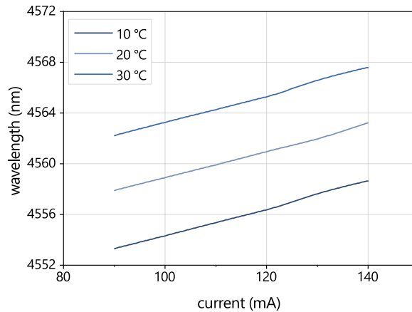
Typical mode hop free tuning of a nanoplus DFB laser at 4565 nm by current and temperature
