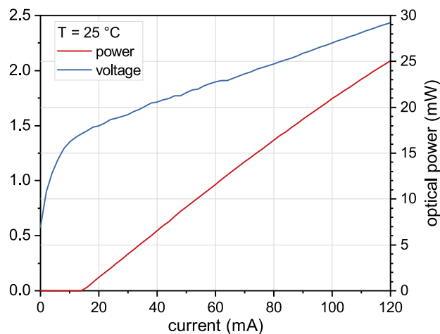
Typical PI and VI curve of a nanoplus FP laser at 1590 nm
