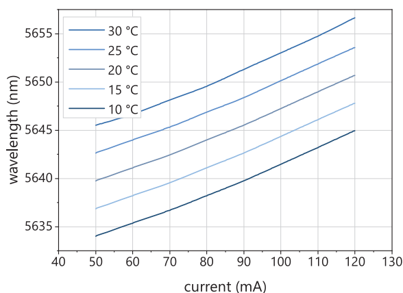
Typical mode hop free tuning of a nanoplus DFB laser at 5645 nm by current and temperature
