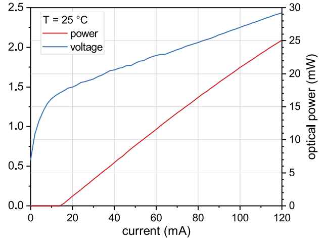
Typical PI and VI curve of a nanoplus FP laser at 1590 nm
